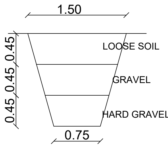
TRIAL PIT NOT TO SCALE
