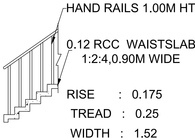
STAIR CASE DETAILS
