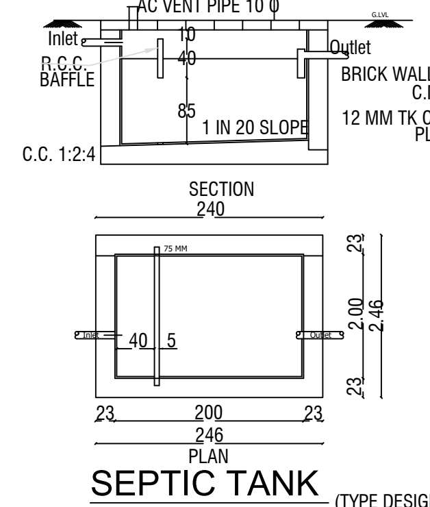
SEPTIC TANK (TYPE DESIGN)
