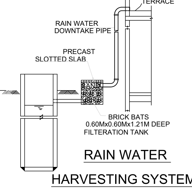
RAINWATER COLLECTION SUMP
