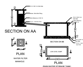
PLAN (RAIN WATER STORAGE TANK)
