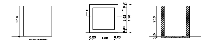
RAIN WATER HARVESTING TANK
