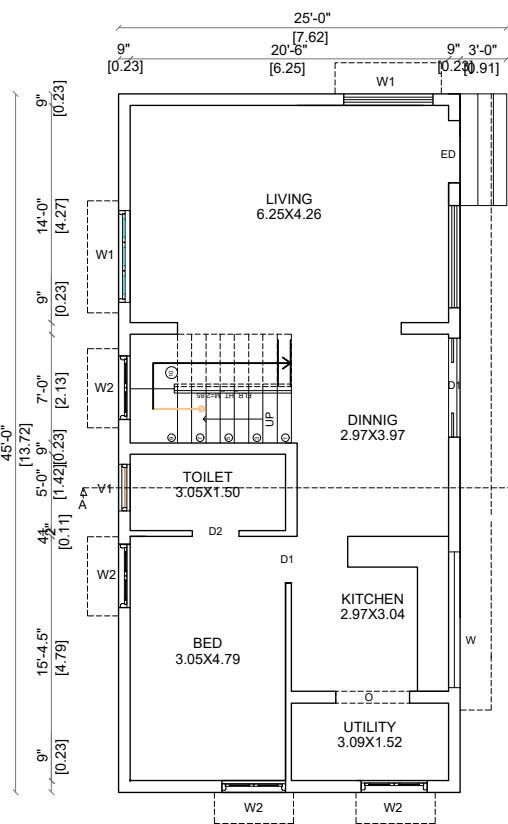
GROUND FLOOR PLAN SCALE: 1"=8'0"
