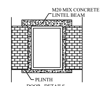
EARTH QUAKE SAFE DESIGN DETAILS
