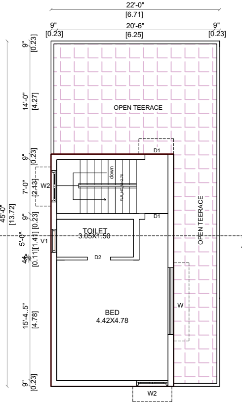
FIRST FLOOR PLAN SCALE: 1"=8'0"
