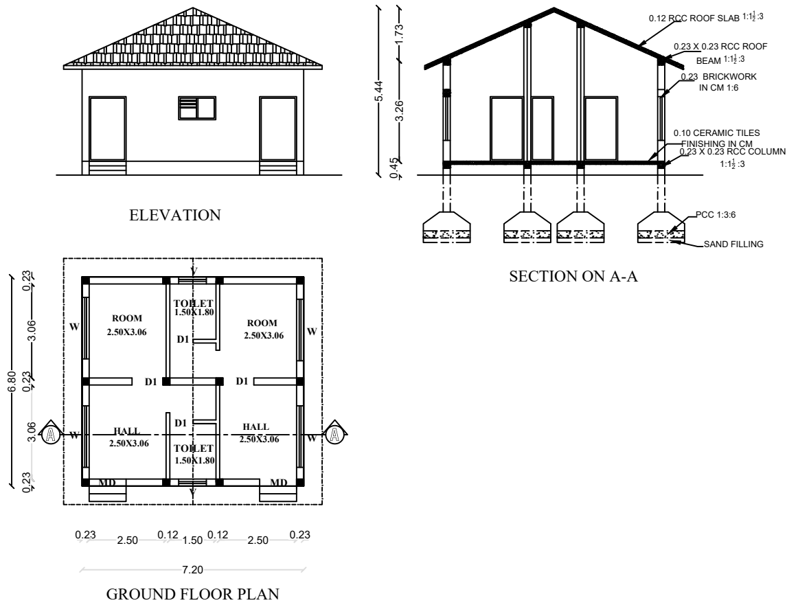
BLOCK 6 - ROOMS
