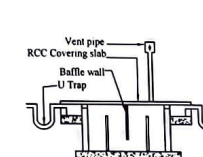
SECTION - 'CD'
