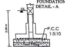
FOUNDATION DETAIL - A
