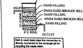
Waste Water Recycle Unit Not To Scale
