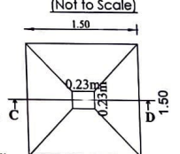
Isolated Footing - A (1.50X1.50)
