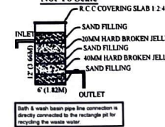
Waste Water Recycle Unit Not To Scale
