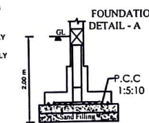
Isolated Footing -A (1.50X1.50) (Not To Scale)
