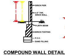
COMPOUND WALL DETAIL
