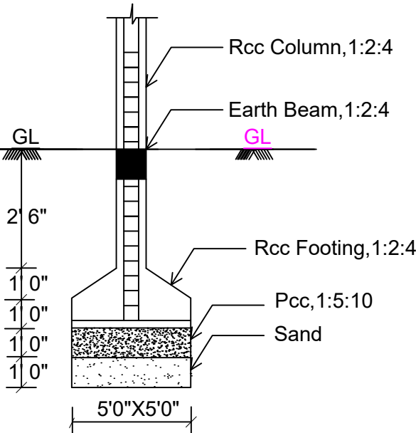
RCC COLUMN DETAILS
