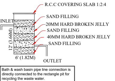
Waste Water Recycle Unit Not To Scale
