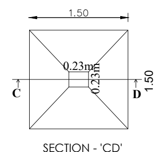
SECTION - 'CD'
