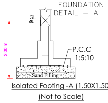
Isolated Footing -A (1.50X1.50) (Not to Scale)
