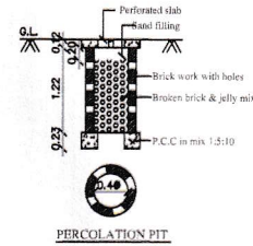
PERCOLATION PIT
