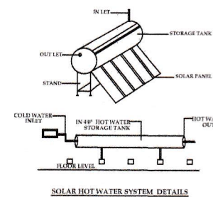
SOLAR HOT WATER SYSTEM DETAILS
