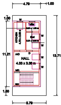
GROUND FLOOR PLAN (NORTH FACING)
