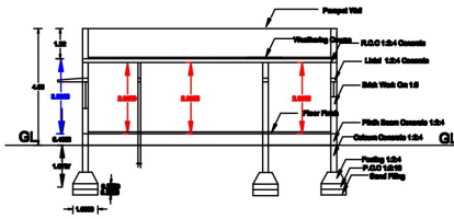
Section Section - AA
