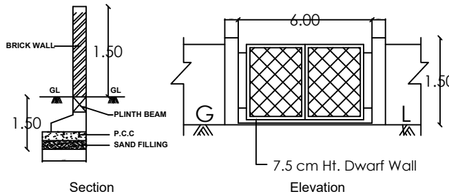
Section
