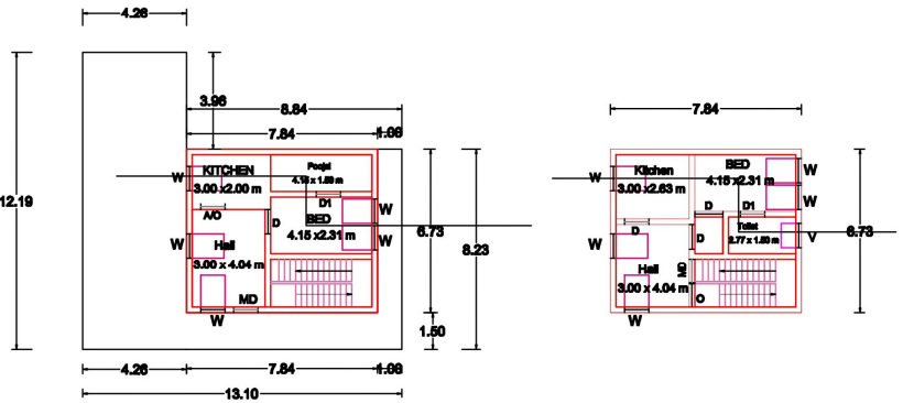
FIRST FLOOR PLAN (North Facing)
