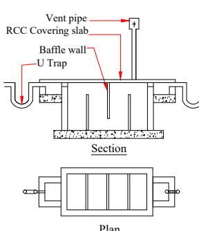
SECTION - 'CD'
