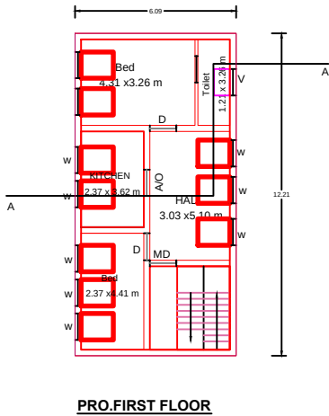
PRO.FIRST FLOOR
