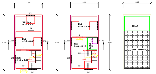
Proposed Ground Floor Plan Proposed First Floor Plan Proposed Terrace Floor Plan
