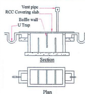
SECTION - 'CD'
