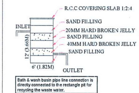
SECTION - 'CD'
