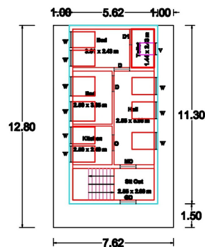
Ground Floor Plan (East Facing)
