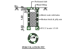
PERCOLATION PIT
