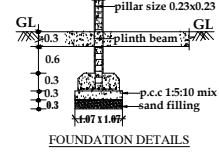
COLUMN FOUNDATION
