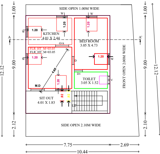
GROUND FLOOR PLAN (NORTH FACING)
