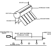
SOLAR HOT WATER SYSTEM DETAILS
