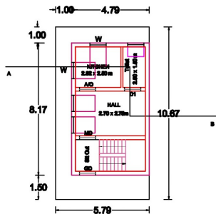
GROUND FLOOR PLAN SOUTH FACING)
