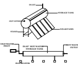
SOLAR HOT WATER SYSTEM DETAILS
