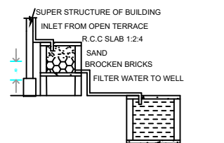
RAINWATER HARVESTING
