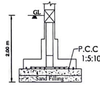
Isolated Footing - A (1.50x1.50) (Not to Scale)
