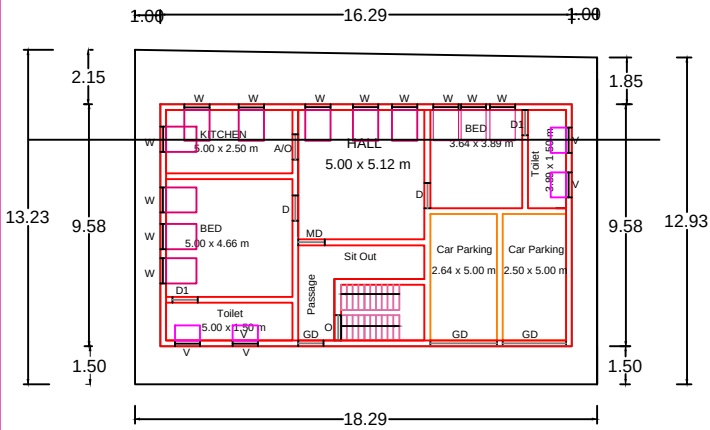
GROUND FLOOR PLAN (NORTH FACING)
