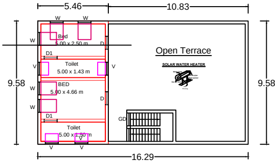
FIRST FLOOR PLAN (NORTH FACING)
