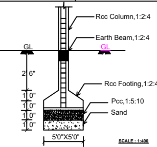
RCC COLUMN DETAILS SCALE : 1:400
