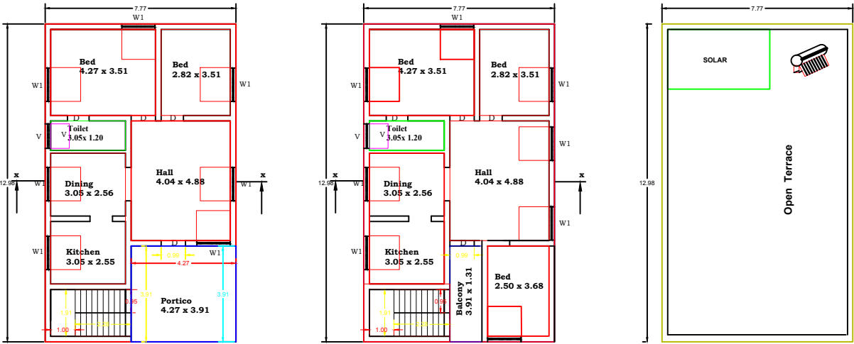
Proposed Terrace Floor Plan
