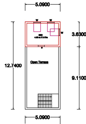
First Floor & Open Terrace
