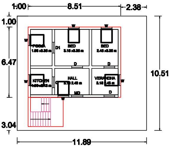
Ex Ground Floor Plan
