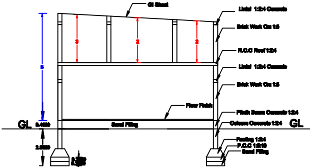
Section Section - AA
