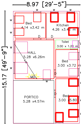
GROUND FLOOR PLAN WEST FACING
