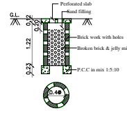
PERCOLATION PIT
