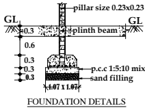
FOUNDATION DETAILS
