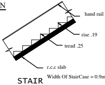
STAIR
