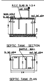
SEPTIC TANK PLAN
