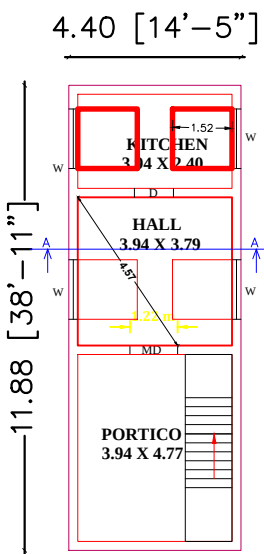
GROUND FLOOR PLAN (WEST FACING)
