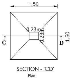
SECTION - 'CD' Plan Using 'U' type trap 2 Nos in inlet, outlet & Ventpipe will be covered with mosquito proof covering net in inner side of vent pipe and top of vent pipe Septic Tank With U Trap Not To Scale
