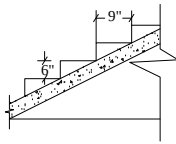
Staircase Detail Not To Scale
