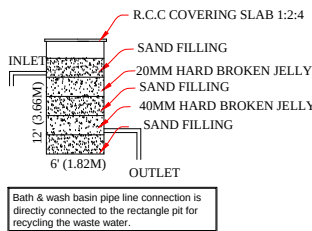
Waste Water Recycle Unit Not To Scale
