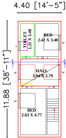
FIRST FLOOR PLAN (WEST FACING)
