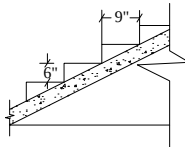
Staircase Detail Not To Scale
