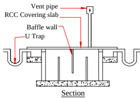
Septic Tank With U Trap Not To Scale Using 'U' type trap 2 Nos in inlet, outlet & Vent pipe will be covered with mosquito proof covering net in inner side of vent pipe and top of vent pipe
