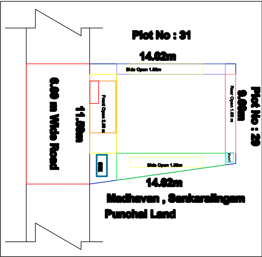
Site Plan
