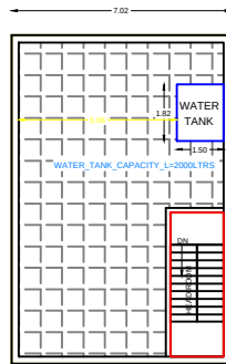
TERRACE PLAN
