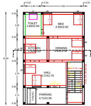
GROUND FLOOR PLAN (Facing North)
