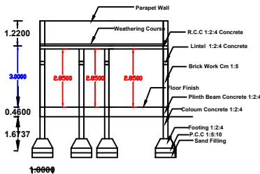
Section Section - AA
