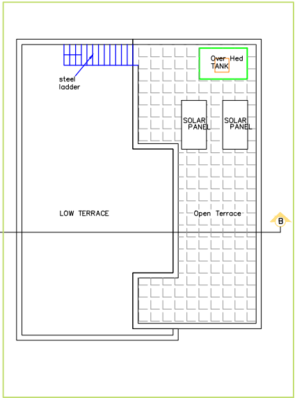
TERRACE FLOOR PLAN BLOC .1
