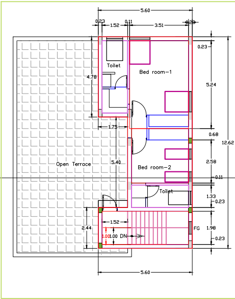
FIRST FLOOR PLAN BLOC .1
