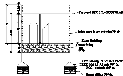
SECTION ON A-A' & FOUNDATION DETAILS
