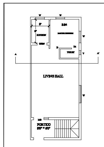
GROUND FLOOR PLAN - NORTH FACING
