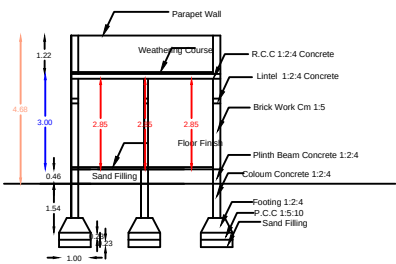
SECTION - AA Section
