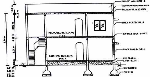
SECTION ON - AB
