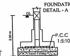
Isolated Footing - A (1.50X1.50)
