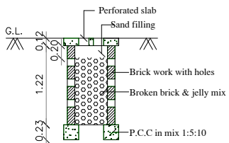
PERCOLATION PIT
