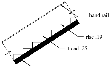
STAIR
