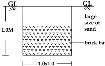
RAINWATER HARVESTING
