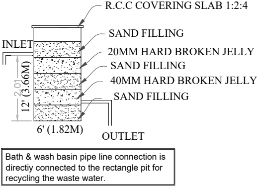
Waste Water Recycle Unit Not To Scale
