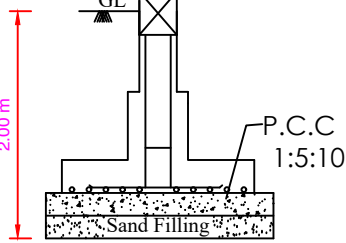
FOUNDATION DETAIL - A
