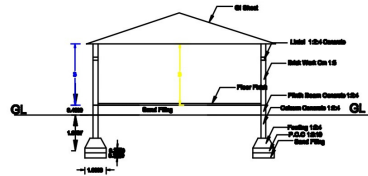
Section Section - AA
