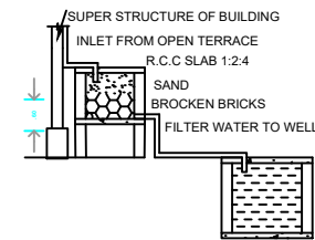
RAINWATER HARVESTING
