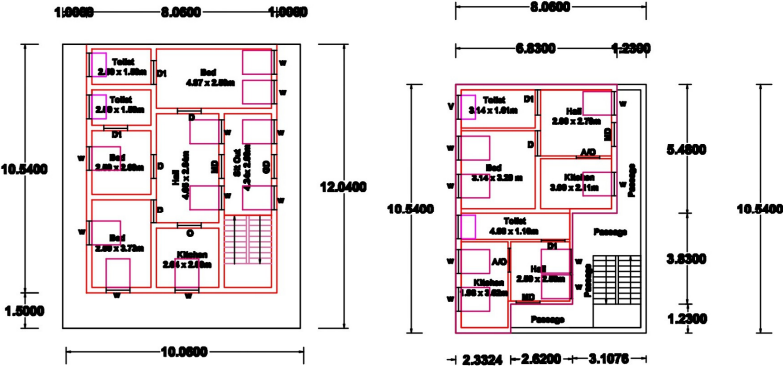
Ground Floor Plan East Facing
