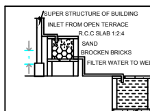
RAINWATER HARVESTING
