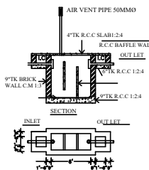
SEPTIC TANK DETAILS SCALE 1"=8'0"
