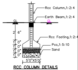
RCC COLUMN DETAILS
