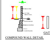
COMPOUND WALL DETAIL
