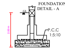
Isolated Footing -A (1.50X1.50) (Not to Scale)
